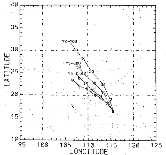
d) DURIAN
